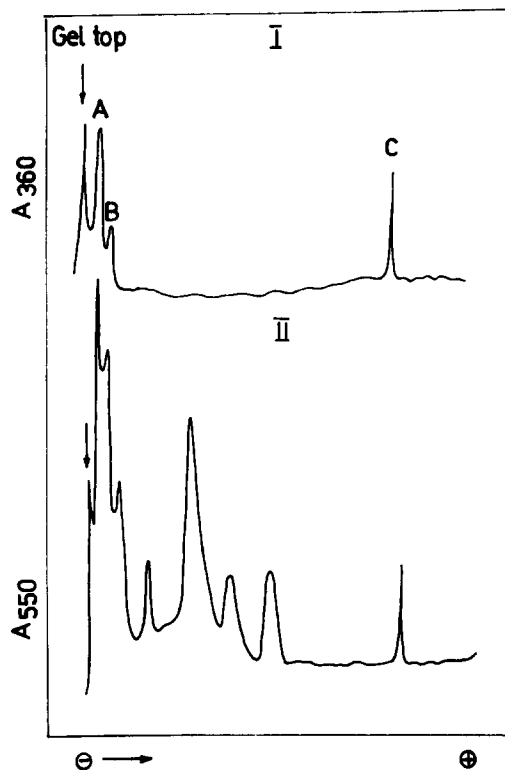
Fig.1. PAGE of the partially purified vacuolar ATPase preparation in non-dissociating conditions. (I) Identification of ATPase by substrate-dependent gel staining with lead acetate; (II) protein staining by Coomassie blue.
